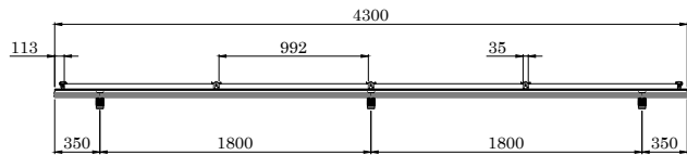
VISTA FRONTAL
